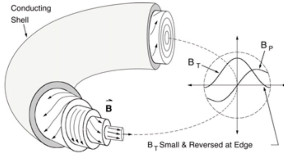
Magnetic Field Structure of the RFP
