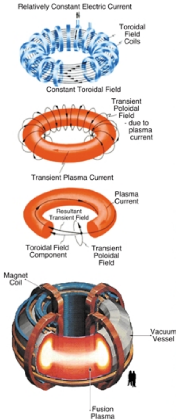
FIGURE 3.1 Components of the tokamak confinement configuration, one of the more advanced plasma confinement concepts. It uses a strong toroidal field created by external field coils (top) to stabilize the plasma while using a poloidal field created by a toroidal plasma current to confine the particles. The final configuration includes a large vacuum vessel to isolate the hot plasma from the surrounding environment (bottom). Courtesy of General Atomics and PPPL.
