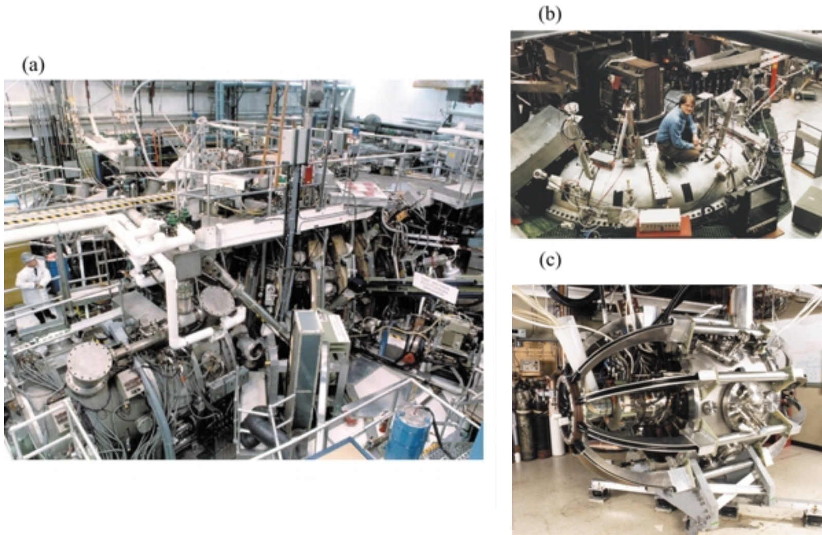
FIGURE 3.6 Examples of the stages of experimental development of plasma configuration concepts: (a) a large advanced tokamak experiment (DIII-D) at the performance extension stage exploring plasma parameters approaching those of a reactor; (b) a mid-sized reversed-field pinch experiment exploring a range of issues at the proof-of-principle stage; and (c) a smaller spherical torus dedicated to exploring a particular type of current drive in a concept exploration experiment. Courtesy of (a) General Atomics, (b) S. Prager (University of Wisconsin at Madison), and (c) T. Jarboe (University of Washington).
