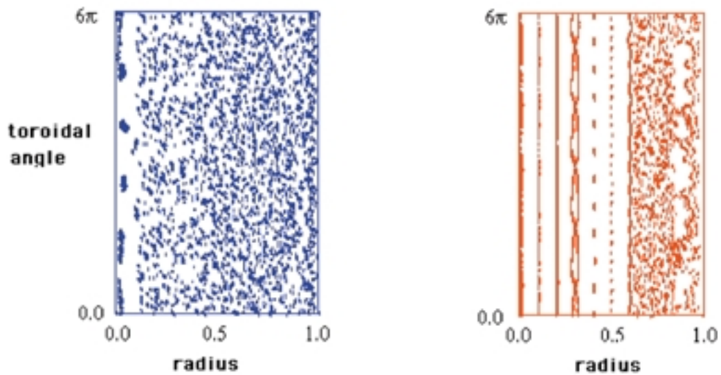
FIGURE 3.3 A magnetic confinement concept such as the reversed-field pinch (top) is a relatively self-organizing configuration that is subject to turbulent magnetic field structures. The magnetic topology includes a reversal of the toroidal field inside the plasma owing to plasma currents. Under normal inductive current drive, the magnetic field lines can readily become chaotic, as indicated by a puncture plot of the field lines as they traverse a poloidal plane (bottom left). With finer control of the plasma currents, well-defined flux surfaces are restored (bottom right). Courtesy of S. Prager (University of Wisconsin at Madison).
